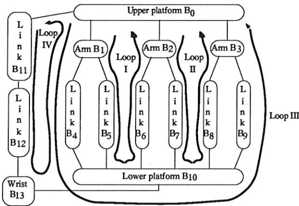
Figure 4 - Sketch of the kinematic loops for the Delta Robot
