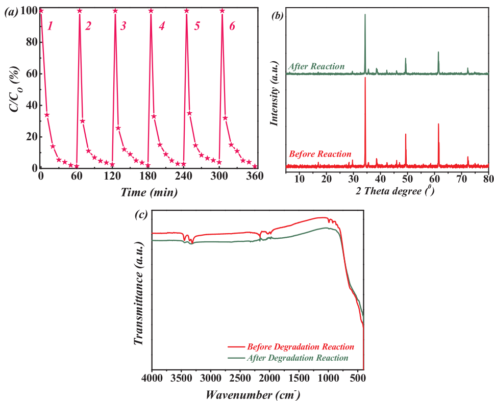
Fig. 5. (a) Six cycle degradations of tetracycline in the presence of octahedron shaped CaCu_3Ti_4O_{12} : catalyst shows high efficiency and stable photolysis even after 360 min visible light irradiation; (b and c) Comparative XRD and FTIR analyses of octahedron shaped CaCu_3Ti_4O_{12} before and after the decomposition experiments over octahedron shaped defective CaCu_3Ti_4O_{12} .
