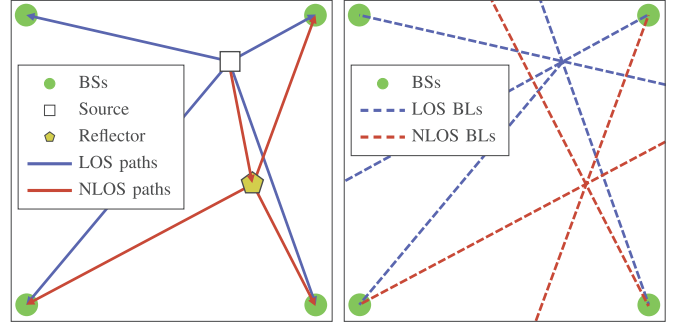
Fig. 2. The left figure plots the LOS and NLOS paths and the right figure plots the bearing lines (BLs). The top left corner base station only receives the LOS path.
