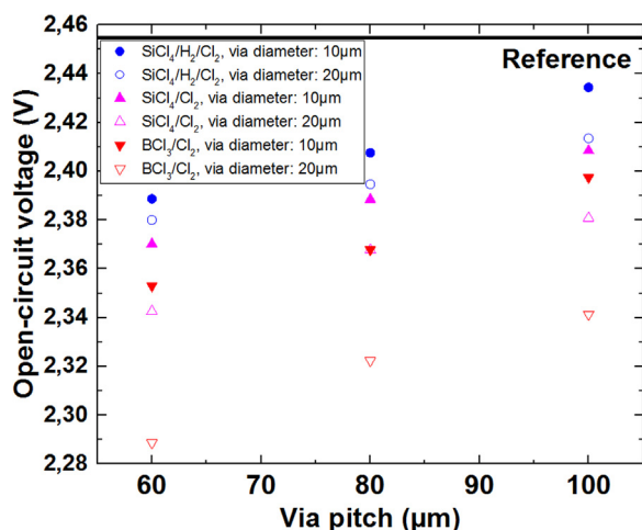
Fig. 6. One-sun open-circuit voltage of the cells with via-holes etched with the three plasma processes as a function of the via pitch. The line corresponds to the V oc of the reference cell without via-holes.
