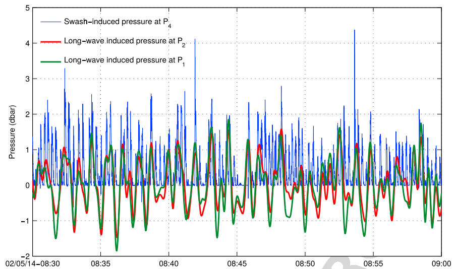
Figure 14. Swash-induced water pressure at P_4 (blue line) and infragravity-wave-induced water pressure at P_1 (green line) and P_2 (red line) on 5 February 2014. The infragravity wave signal was obtained by low-pass (0–0.035 Hz) filtering the pressure signal.
