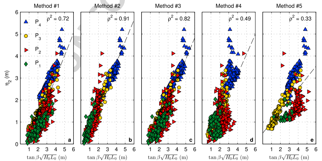
Figure 11. Scatter diagrams of \eta_2 versus \tan \beta \sqrt{H_0 L_0} , with \tan \beta the foreshore slope computed with method 1 to 5 (a–e). The squared correlation coefficients computed for the whole data set are indicated on the top right hand corner.
