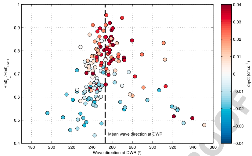
Figure 6. Scatter diagram of the ratio Hm0_{P_0}/Hm0_{DWR} versus the wave direction measured at DWR. The color scale represents the gradient of elevation and indicates the tidal stage (red for flood and blue for ebb). The black-dashed line indicates the average mean wave direction at DWR. DWR = Datawell DWR-MkIII.
