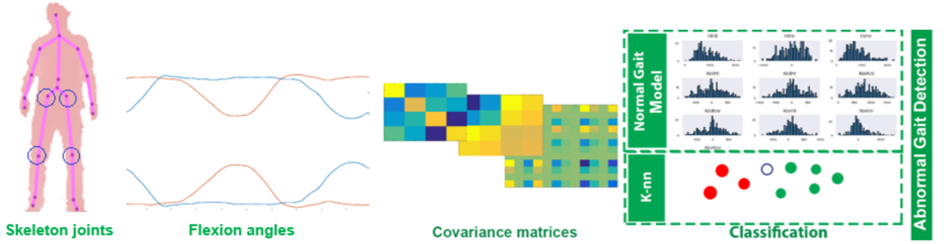
Fig. 1. The proposed binary gait assessment pipeline. We select the most stable among low-limbs skeleton joints to calculate flexion angles. Then the angles-based covariance features are used for gait assessment in different scenarii.
