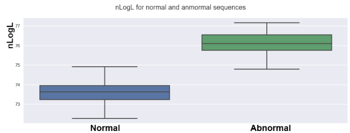
Fig. 3. The nlogL for normal/abnormal gait sequences from [7] by the pdf(cov) build on the [11] dataset. The resulting distribution and confidence intervals show that the data are easily separable.
