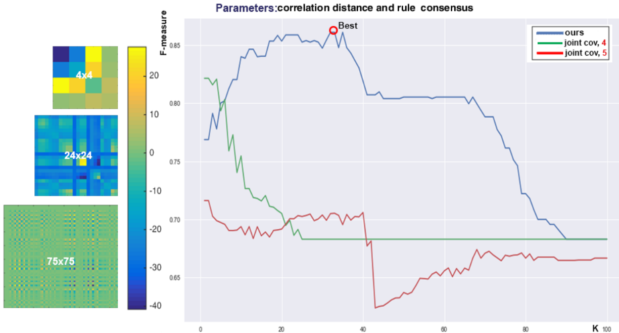
Fig. 2. Curves for results summarized in Table III and corresponding covariance matrices.
