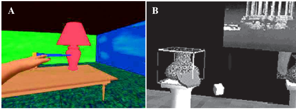
Fig. 1. A) Ray casting technique [3] B) Go-go technique [10]
