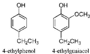
Fig. 1. Structures of 4-ethylphenol and 4-ethylguaiacol.
