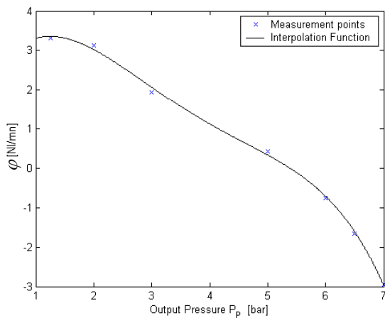
Figure 6. Approximation of mass flow rate measured for U_i = 0 : Function \phi(p)
