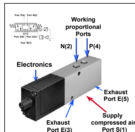
Figure 1. Photograph and schema of a FESTO MPYE-5-M5-010B proportional valve
