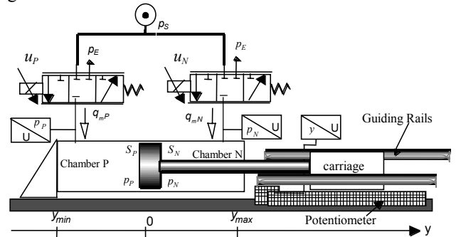
Fig.5. The electropneumatic system
