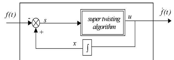
Fig.1. The structure of the differentiator
