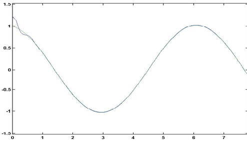
Fig.3. Derivative of signal in the presence of a noise: robust differentiator
