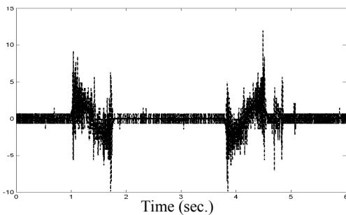
Fig. 7. Acceleration and desired acceleration ( \text{ms}^{-2} )
