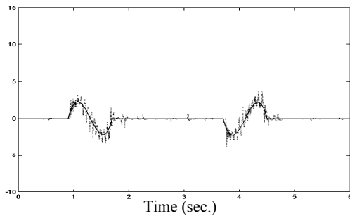
Fig.10. Acceleration and desired acceleration ( \text{ms}^{-2} )
