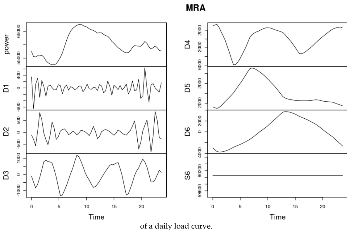
Figure 5. Multiresolution analysis of a daily load curve.
