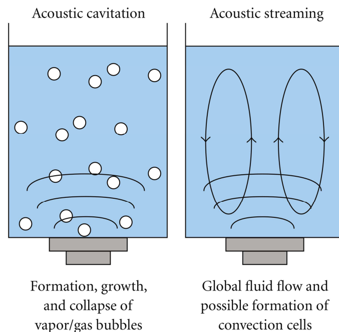
Fig. 1: Illustration of ultrasonic cavitation and acoustic streaming effects as presented in [19]
