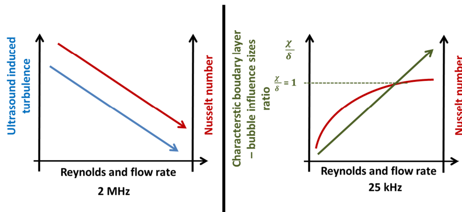
Fig. 15 : Illustration of the phenomenon involved in heat transfer enhancement by ultrasound in presence of acoustic streaming (2 MHz) and acoustic cavitation (25 kHz).
