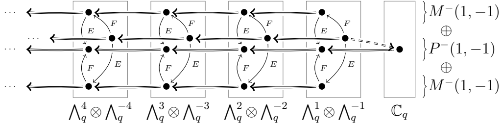
Figure 2: The two commuting actions of (7.17).
