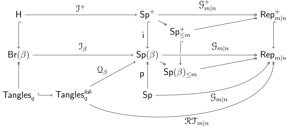
Figure 1: Overview of the categories and functors involved in our construction. (The third column makes sense only for \beta = m - n .)
