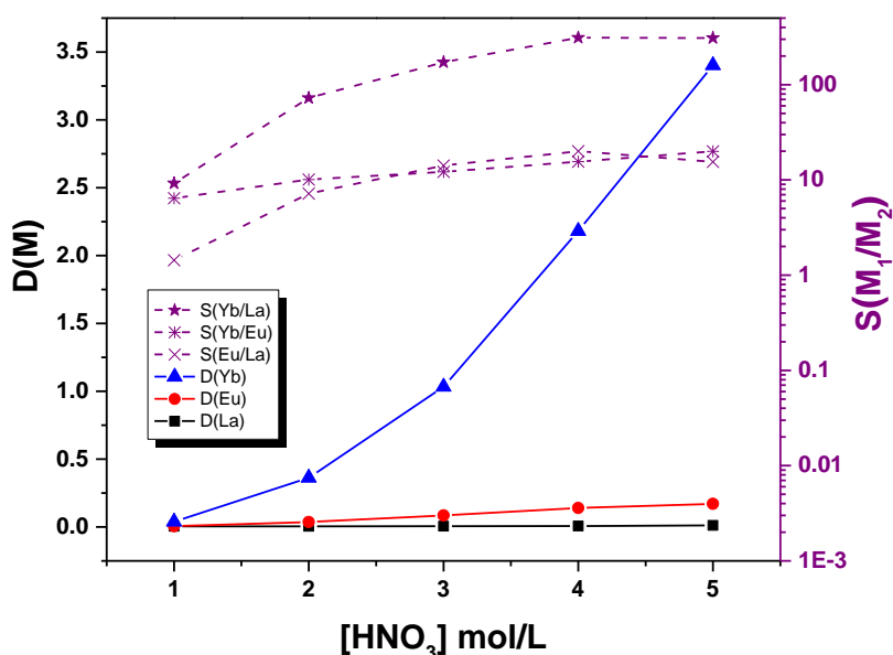
Figure 4: Effect of nitric acid concentration on the Distribution ratios and the selectivity factors of La(III), Eu(III), and Yb(III); Organic phase: 1 mM CR4-Tz-DODGA in toluene / iso-octanol (90/10 v/v); Aqueous phase: 1 mM \text{Ln}(\text{NO}_3)_3 in 1 – 5 M \text{HNO}_3 .
