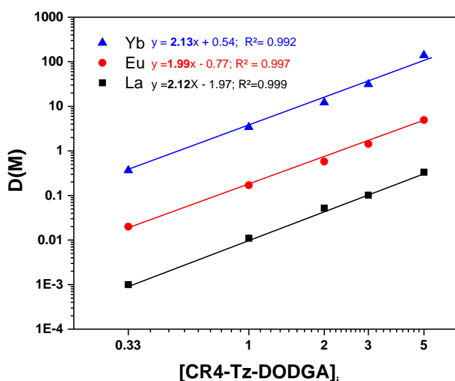
Figure 5: Effect of the extractant concentration on the distribution ratios of Ln(III); Organic phase: 0.33-5 mM CR4-Tz-DODGA in toluene / iso-octanol (90/10 v/v); Aqueous phase: 1 mM Ln(NO 3 ) 3 5M in HNO 3 .
