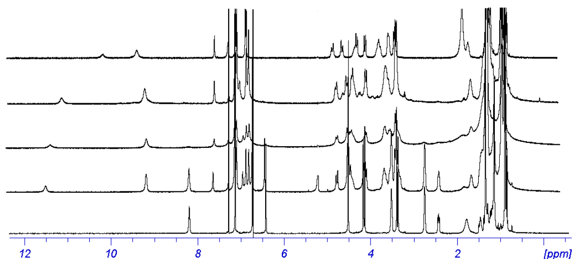
Figure 7: NMR titration spectra of the ligand NOCAC with \text{UO}_2(\text{NO}_3)_2 at different ratios varied from [\text{NOCAC}]/[\text{UO}_2^{2+}] = 1:0 to 1:2 , [\text{NOCAC}] = 30 \text{ mM} in \text{CDCl}_3 .
