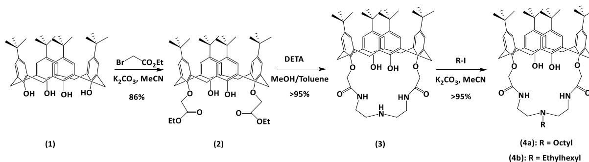
Figure 1: Synthetic scheme for NOCAC ( 4a ) and NEHCAC ( 4b ).
