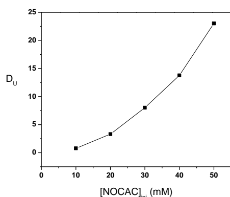
Figure 3: Effect of the extractant concentration on the distribution ratios of U(VI). Organic phase: NOCAC 10–50 mM in dodecane/octanol (83/17 v/v); aqueous phase: 1 mM \text{UO}_2(\text{NO}_3)_2 in 0.1 M \text{H}_2\text{SO}_4 . A/O = 1.
