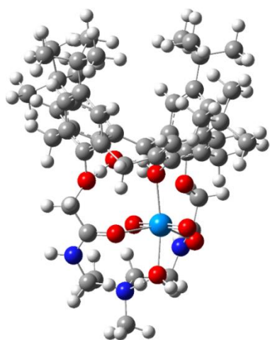
Figure 9: Structure obtained by DFT calculations on the U-NOCAC complex.
