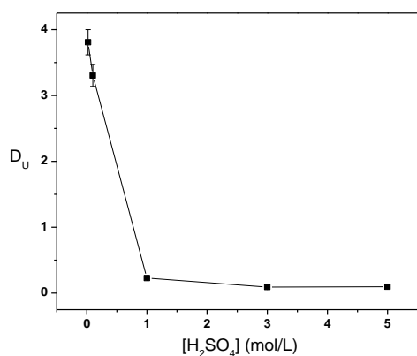
Figure 2: Effect of feed sulfuric acid concentration (0.02–5 M) on the distribution ratio of \text{UO}_2^{2+} . Organic phase: 0.02 M NOCAC in dodecane/octanol (83/17 v/v); aq. phase: 1 mM \text{UO}_2(\text{NO}_3)_2 in \text{H}_2\text{SO}_4 . Aqueous to organic ratio (A/O) = 1.
