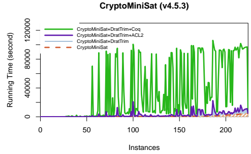
Fig. 16. Benchmark of [Cruz-Filipe et al. 2017a]
