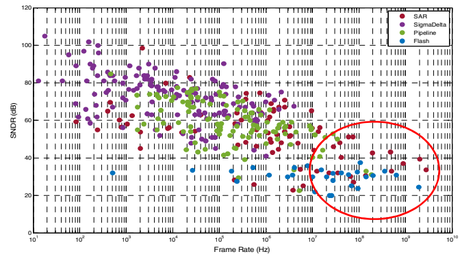
Fig. 3. State of the art of 8-bit ADC from [9]. At the targeted frame rate, SAR architecture offers the best signal to noise ratio.
