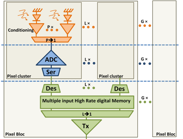
Fig. 2. IC repartition of a 3D CMOS stacked BIS. The first tier is for the pixel frontend, the second tier shares one ADC for one pixel clusters and the third tier is for the deigital memory shared for several ADC clusters.
