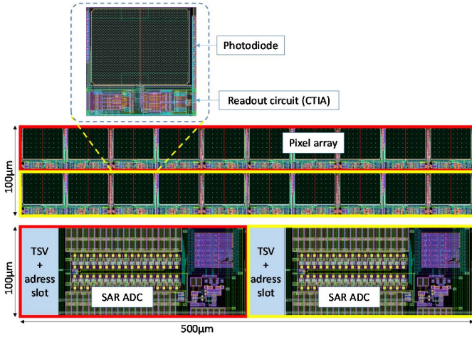
Fig. 4. tier 1 (top) and tier 2 (bottom) floorplan partitioning ( 100\mu\text{m}\times 500\mu\text{m} double cluster)
