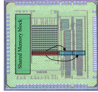
Fig. 5. Demonstrator die photography. Highlighted: two clusters of 10 pixel (pink) and their two associated ADCs (blue) and the shared memory bank for the block of 12 digital clusters.
