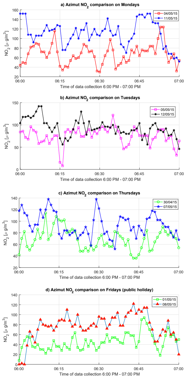
Figure 8: Daily comparison of \text{NO}_2 concentrations.
