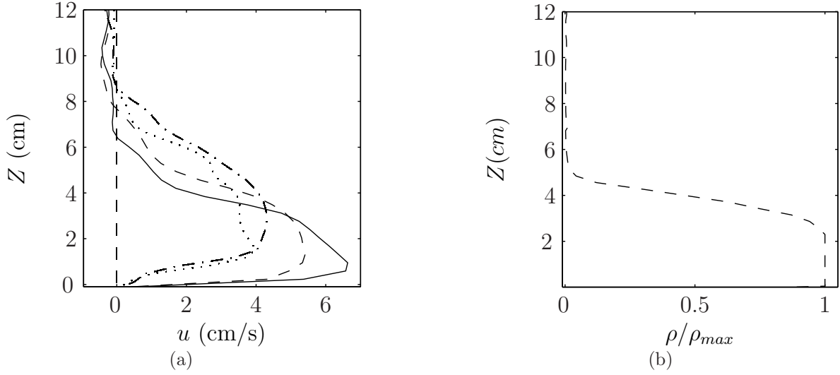
Figure 2: Initial conditions of the gravity current flowing on the initial horizontal channel. (a) Mean velocity profiles at X = 20\text{cm} (....), 85 (---), 195\text{cm} (— · —) and 199\text{cm} (—) from the gate; (b) vertical density profile obtained from the dye visualizations at D = 195\text{cm} from the gate for experiment C3.
