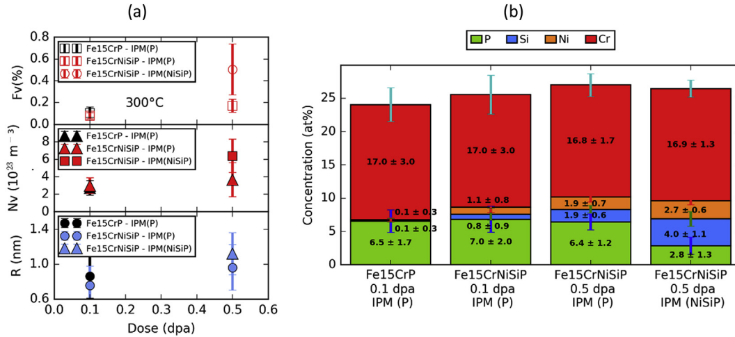
Fig. 7. Cluster characteristics of ion-irradiated specimens at 300 °C as a function of the dose a) volume fraction (Fv), number density (NV) and radius (R) of the SRCs, b) solute concentration of the clusters. Fe concentration makes the balance to 100%.
