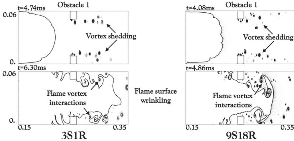
Fig. 7. Numerical Schlieren ( \nabla \rho/\rho ) and isocontour of progress variable c = 0.5 showing the flame interaction with the first obstacle. Left: single-step mechanism. Right: Multi-step mechanism.
