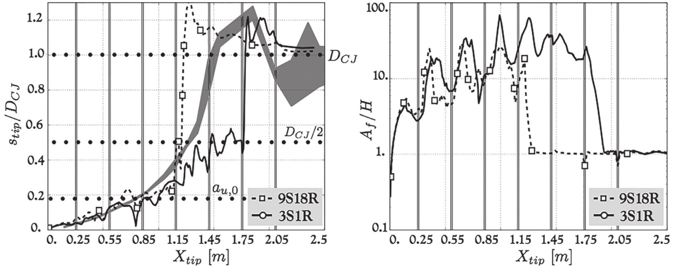
Fig. 6. Evolution of the non-dimensional flame tip speed (left) and non-dimensional flame surface (right) with the flame tip position. The gray area represents the experimental shots. The vertical bars represent the position of the seven obstacles. a_{u,0} is the sound speed at the fresh gases for the initial conditions.
