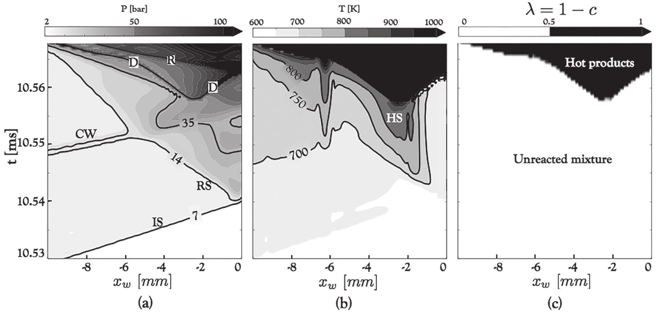
Fig. 13. Time evolution of pressure (a), temperature (b) and \lambda = 1 - c (c) in the single-step case through the cut line presented in Fig. 10(Right), positioned 500 \mu\text{m} from the bottom wall. x_w is the distance from the obstacle 6 left wall. IS , RS , CW , R and D denote an incident shock, a reflected shock, a compression wave, the retonation wave and the detonation wave, respectively. HS is a hot spot.
