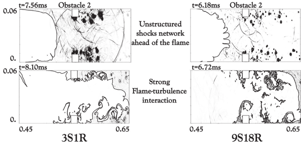
Fig. 8. Numerical Schlieren ( \nabla\rho/\rho ) and isocontour of progress variable c = 0.5 showing the shocks network formed ahead of the flame. Left: single-step mechanism. Right: Multi-step mechanism.
