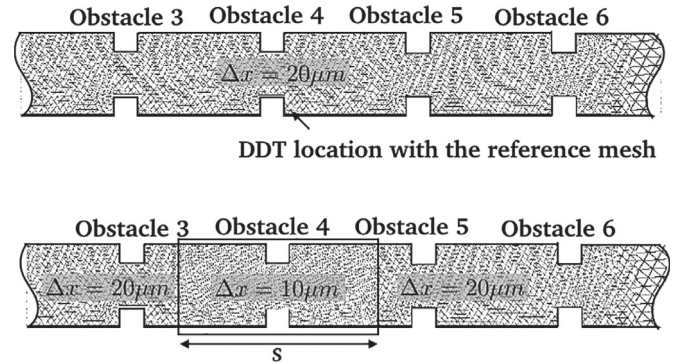
Fig. 17. The meshes used to perform the grid independence study in the multi-step chemistry case. (Top) Reference mesh, used in the core of the manuscript, where the smallest cell size is 20\ \mu\text{m} . (Bottom) A new mesh with a higher resolution window, 300\ \text{mm} large, centered around the DDT location (just after obstacle 4) and where the cell size is 10\ \mu\text{m} .
