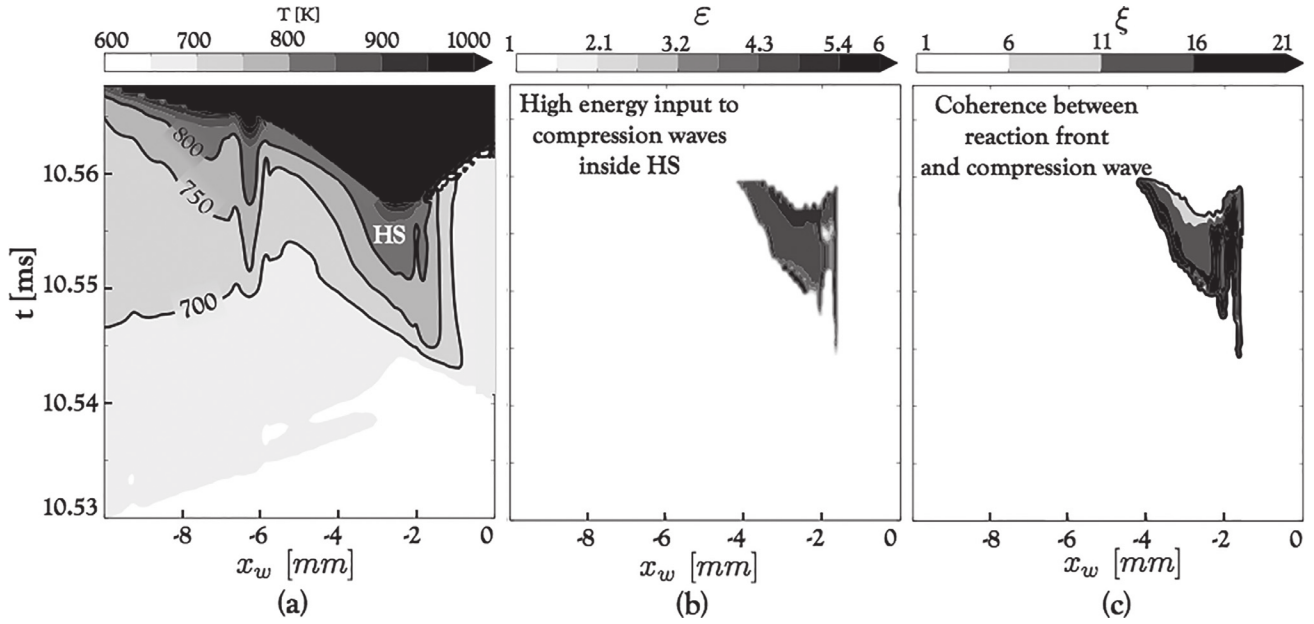
Fig. 14. Time evolution of temperature (a), \varepsilon (b) and \xi (c) in the single-step case through the cut line presented in Fig. 10(Right), positioned 500 \mu m from the bottom wall. x_w is the distance from the obstacle 6 left wall. IS, RS, CS, R and D denote an incident shock, a reflected shock, a compression wave, the detonation wave and the detonation wave, respectively. HS is a hot spot.
