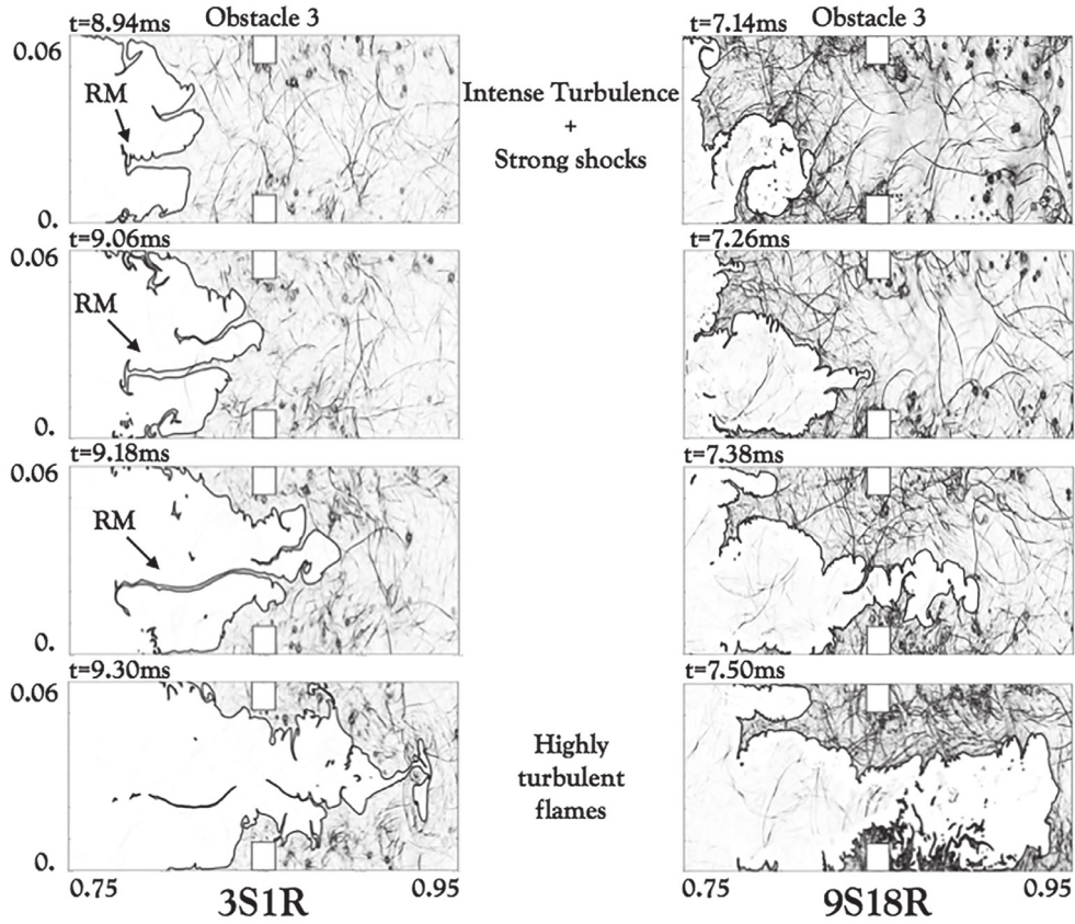
Fig. 9. Numerical Schlieren ( \nabla\rho/\rho ) and isocontour of progress variable c = 0.5 showing the highly turbulent flame crossing the third obstacle. RM denotes the Richtmyer-Meshkov (RM) instability. Left: single-step case. Right: multi-step case.
