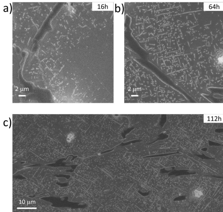
Figure 4: SEM images (secondary electron detector) showing the microstructure of steel 2 (etched using oxalic acid solution to brightly image carbides) after aging at 750^\circ\text{C} during 16 h (a), 64h (b) and 112h (c). Precipitation of M_{23}C_6 secondary carbides in the vicinity of primary carbides is clearly exhibited for the early stage of aging, and it progressively extends in the matrix.
