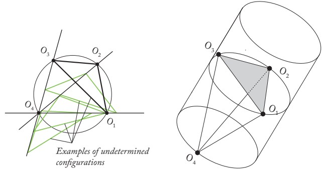
Examples of undetermined configurations (a) in SE(2) , when all agents belong to the same circle (gained finite motion, also called self motion)
