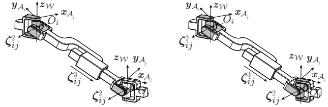
Fig. 3. Virtual kinematic chains corresponding to the elementary edges for \mathbb{R}^3 \times \mathcal{S}^1 . The dark-gray joints are the actuated joints.
