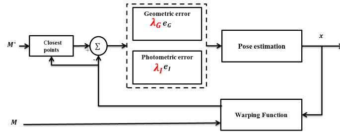
Figure 1. Classic hybrid approach diagram. The geometric and photometric error ( e_G and e_I , respectively) are jointly minimized. A tuning parameter \lambda = (\lambda_G, \lambda_I) weights the contribution of each measurement during the minimization process. The metric measurements are represented in a i -th single vector \mathbf{M}_i = [\mathbf{P}_i^T \ \mathbf{I}_i]^T \in \mathbb{R}^4 , which contains the 3D Euclidean points \mathbf{P} and its associated intensities \mathbf{I} .
