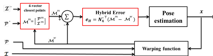
Figure 4. Point-to-hyperplane approach diagram. In the first iteration, the closest points can be estimated by finding in a kd -tree with the 4D vector and linear interpolation in the following iterations. The method is invariant to a tuning parameter \lambda .
