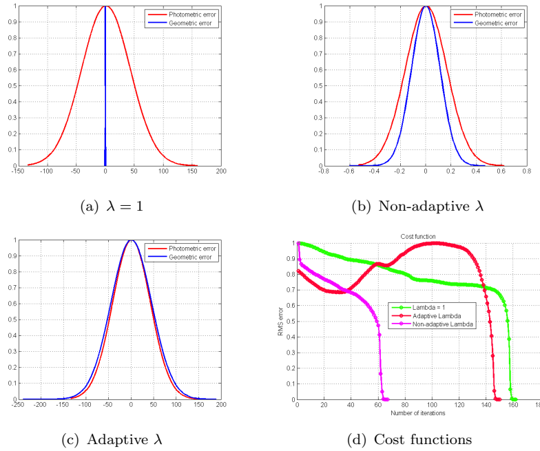
Figure 3. Influence of the scale coefficient on the error function residuals (Equation (13)) when (a) \lambda is not estimated, (b) when the intensities and 3D points are normalized between [0, 1] [18] and (c) when \lambda is estimated at each iteration [15]. An example of a cost function is shown in (d), which indicates that the number of iterations can be improved when a good choice of \lambda is made.
