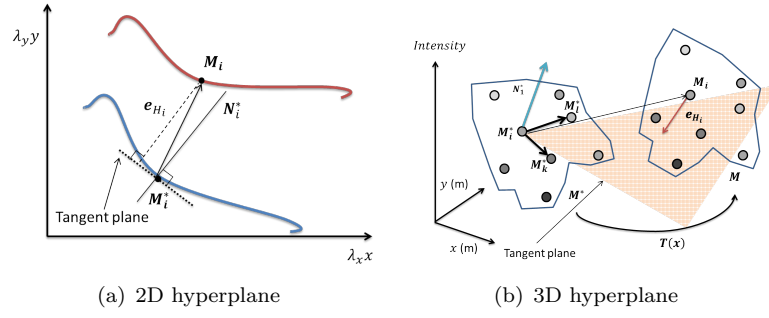
Figure 5. Principle of the Point-to-hyperplane applied in 2 dimensions Point-to-line and 3 dimensions Point-to-plane. It should be noted that the axis x and y are not in the same scale in (a). A tuning parameter \lambda is added in order to demonstrate the invariance of the Point-to-hyperplane method in the 2D case. The distance e_{H_i} is the result of projecting the vector \overrightarrow{M_i^* M_i} onto the normal direction N_i^* .
