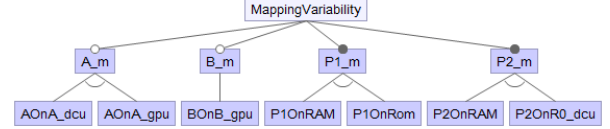
(a) Mapping FD
