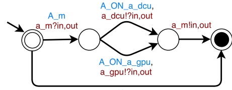
(c) Task Mapping A FA
