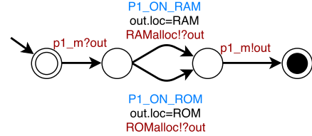
(b) data-path Mapping p1 FA
