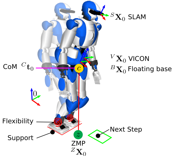
Fig. 4. This HRP-4 is fitted with a passive mechanism between its ankles and feet soles, which provides a spring-damper compliant system. Its state is taken into account by estimating the robot’s floating base with dense visual SLAM and validated with a VICON tracking system, with reflective IR markers attached to the floating base link. The ZMP is estimated from ankle force-torque sensors. Note that here it is depicted outside of the robot’s support polygon and triggers a step from the MPC.
