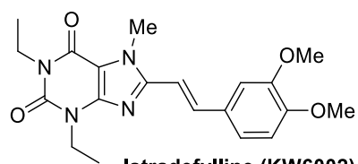
Istradefylline (KW6002)
