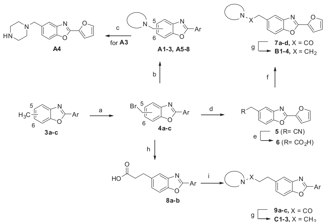
Scheme 2. Reagents and conditions: (a) NBS, benzoyl peroxide, CCl 4 , reflux/hν (230 W), 60–75%; (b) R 2 R 1 NH, Et 3 N, acetone, 50–85%; (c) TFA, DCM, 60%; (d) KCN, EtOH/H 2 O, 50–60%; (e) H 2 O/H 2 SO 4 /AcOH, reflux, 60–70%; (f) i ) SOCl 2 , toluene; ii ) secondary amine, Et 3 N, EtOAc, 50–60%; (g) LiAlH 4 , THF, 60–75%; (h) i ) dimethyl malonate, K 2 CO 3 , acetone; ii ) NaOH, H 2 O then 6 M HCl; iii ) DMF, reflux, 40–43%.
