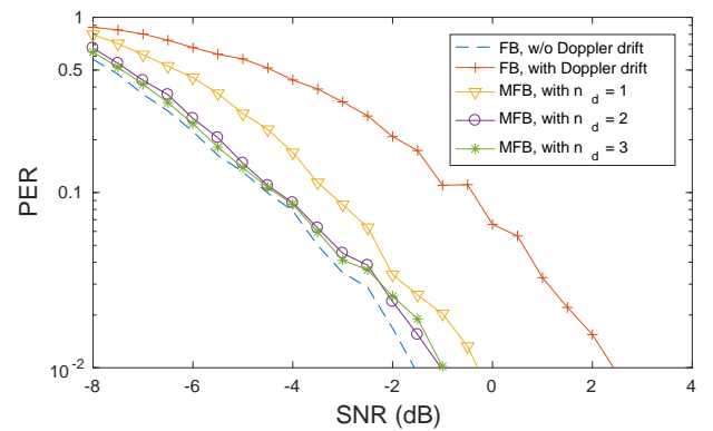
Fig. 6: Performance of different detection methods.
