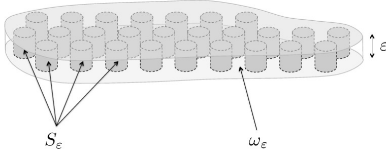
Figure 1: Views of the domain \Omega_\varepsilon
