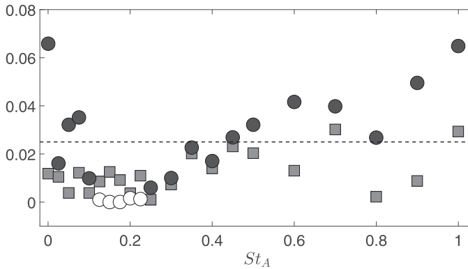
FIG. 7. Mass balance along the mean recirculation region. Symbols: ■ |\epsilon_R^*| ; --- |\epsilon_R^*| = 0.025 ; ○ \dot{m}_R^* . Empty symbols indicate points for which |\epsilon_R^*| < \dot{m}_R^* .
