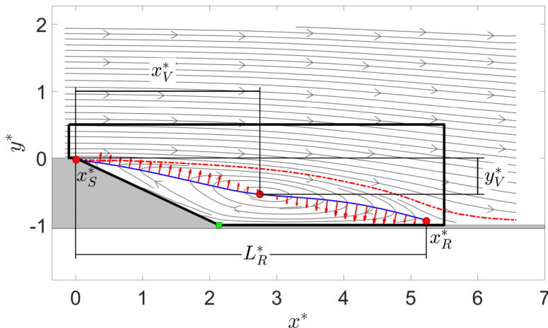
FIG. 1. Streamlines of the baseline separated flow. Symbols: \text{---} (gray online) streamlines; \text{—} (black online) closed contour S_V , used for the computation of \Gamma^* ; \text{—} (blue online) mean separation line; \text{- - -} (red online) separating streamline; \bullet mean separation point (x_S^*, 0) , center of the vortex (x_V^*, y_V^*) , and mean reattachment point (x_R^*, -1) ; \blacksquare position of the pressure tap measuring P_b (see Sec. VI). Red arrows represent mass fluxes [V \cos(\phi)] through the mean separation line.
