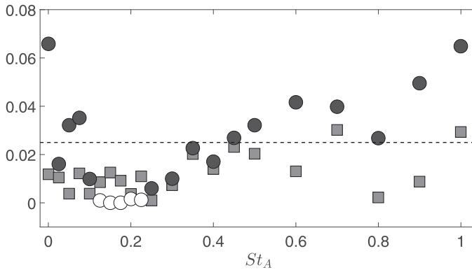
FIG. 7. Mass balance along the mean recirculation region. Symbols: \blacksquare |\epsilon_R^*| ; -\text{---} |\epsilon_R^*| = 0.025 ; \circ \dot{m}_R^* . Empty symbols indicate points for which |\epsilon_R^*| < \dot{m}_R^* .
