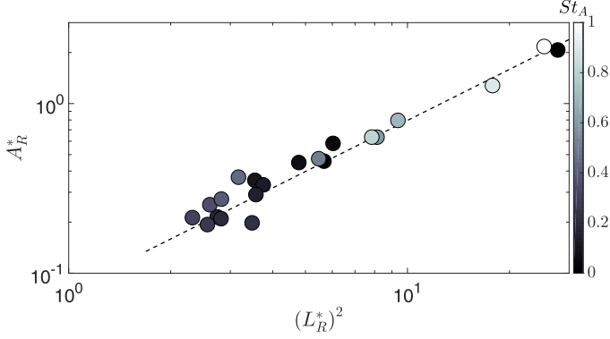
FIG. 6. Correlation between A_R^* and (L_R^*)^2 . The grayscale indicates the value of St_A , and the dashed line (— — —) represents a best fit of Eq. (12) on available data. Log-log representation is used to highlight scatter for small values of (L_R^*)^2 .
