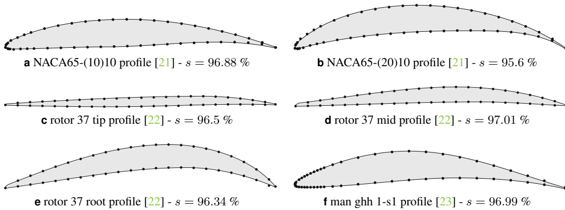
Figure 8. superimposition of 6 compressor blade profiles as given in the literature (●) and the associated parameterized profiles (□)
