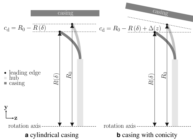
Figure 3. effect of casing conicity on the computation of dynamic clearance, blade at rest (—) and vibrating blade (—)
