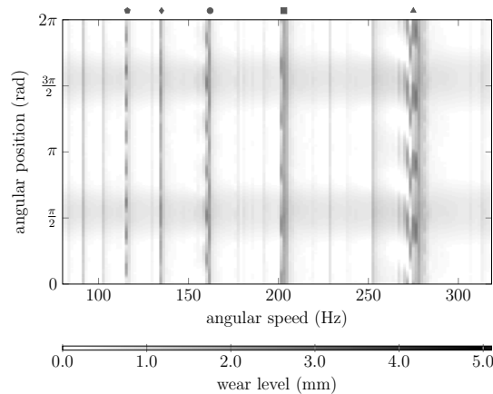
b wear map
