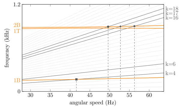
a Campbell diagram
