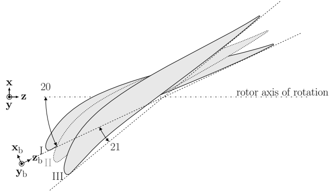
(20) angle of incidence (21) stagger angle
