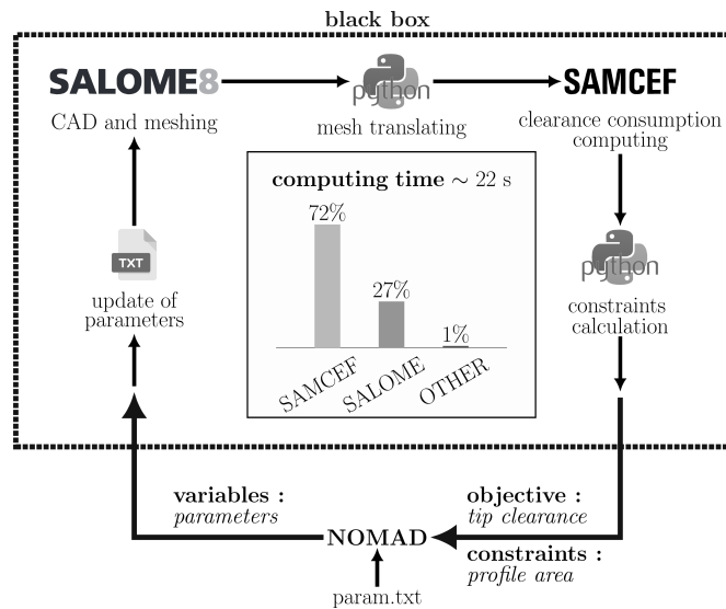
Figure 11. description of one iteration of the procedure
