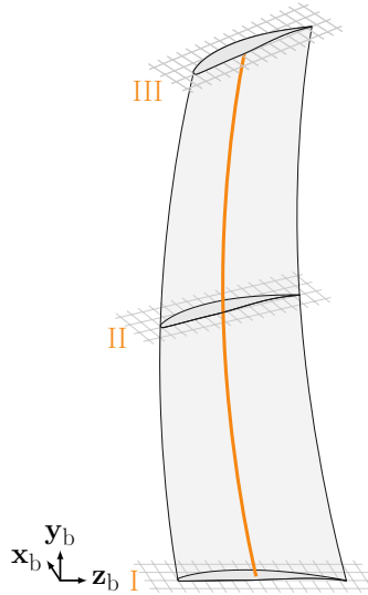
Figure 4. blade model with associated profiles (□) and stacking line (—)
