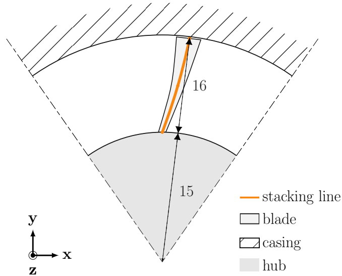
a rear view of the blade/hub assembly within a casing
