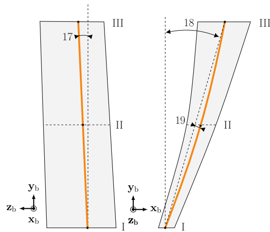
b side view of the blade
