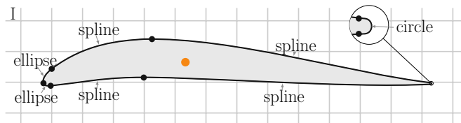
Figure 5. profile description with center of gravity (●)
