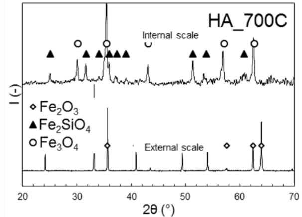
Figure 8: X-Ray diffractograms of internal and external scales on HA_700C sample.
