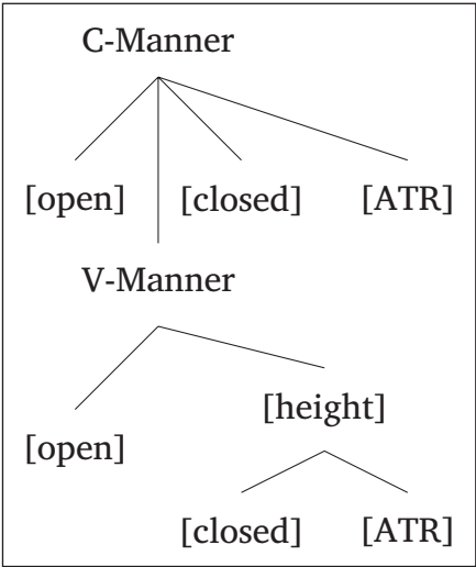
Figure 3: Modified PSM – Manner features.
