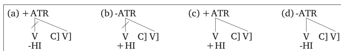
Figure 1: Spreading and delinking (Hantgan & Davis 2012).
