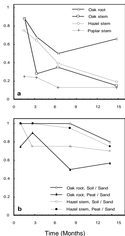
Fig. 1. Survival of Collybia fusipes on several kinds of wood segments buried in soil. a, experiment 1; b, experiment 2. Wood segments were incubated 4.5 months in experiment 1 and 10 months in experiment 2 before being buried in soil
