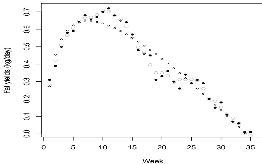
Fig. 1 Semiparametric regression estimation for average daily fat data. The points in black represent the observed data, the circles in grey represent the semiparametric binomial kernel regression estimator with Bayesian bandwidth and the circles in black represent the GLM.
