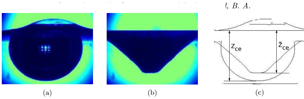
Figure A.12: (a) Static bubble of R = 2.15\text{mm} in water; (b) the conical cavity just before jet formation in the same bubble; (c) the shape contours extracted from (a) and (b) are superposed together to show the displacement of the bottom of the cavity.
