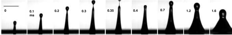
(b) R = 0.81\text{mm} ( Bo = 0.11 , Oh = 2.21 \times 10^{-2} ) in GW48 ( 20^\circ\text{C} ). The line in image is 0.5mm. d_j/R \approx 0.04 .
