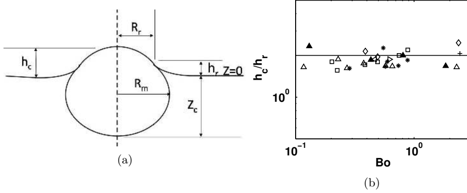
Figure 3: (a) Schematic of the static bubble shape; (b) h_c/h_r as a function of Bo . \Delta , Water; \triangleright , GW48 (20°C); \blacktriangle , GW48 (30°C); * , GW68; \diamond , GW72; \triangleleft , ethanol; + , 2-propanol; —, h_c/h_r = 2 .
