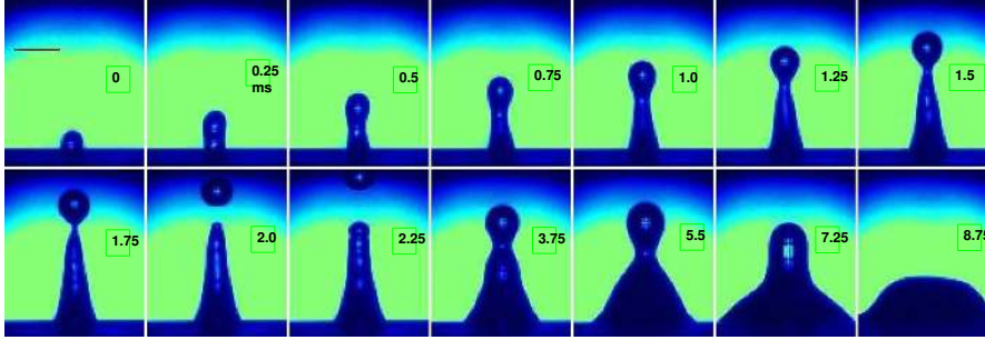
(a) R = 4.08\text{mm} ( Bo = 2.25 , Oh = 1.85 \times 10^{-3} ). The grid size in the image is 1mm. d_j/R \approx 0.32 .
