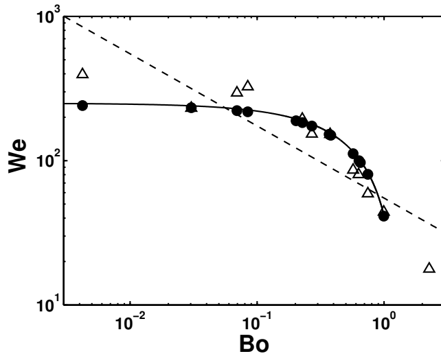
Figure A.14: Comparison of the jet Weber number measured by two methods plotted against Bo . \Delta , We based on jet velocity at free surface; \bullet , We_{jc} based on jet velocity measured as U_{jc} = \tilde{Z}_{ce}/t_j , where t_j = 0.11t_c from figure A.13b and \tilde{Z}_{ce} = 0.86 Z_{ce} ; - -, We = 55 Bo^{-1/2} ; —, We = 62.5(Z_{cd}/R)^2 .
