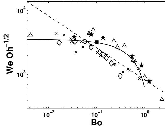
Figure 9: Variation of the Weber compensated for capillary wave damping with Bo . Symbols are the same as in figure 5. - -, We Oh^{-1/2} = 830 Bo^{-1/2} ; —, We Oh^{-1/2} = 900 (Z_{cd}/R)^2 .
