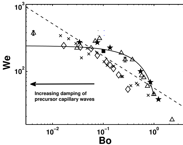
Figure 5: Variation of jet Weber number with Bond number in water. \triangle , present experiments; \star , BSB; \diamond , drop velocities of Spiel (1995); \blacksquare , Kientzler et al. (1954); —, We = 62.5(Z_{cd}/R)^2 ; - -, We = 55 Bo^{-1/2} ; \times , jet velocities of Ghabache et al. (2014) for water.
