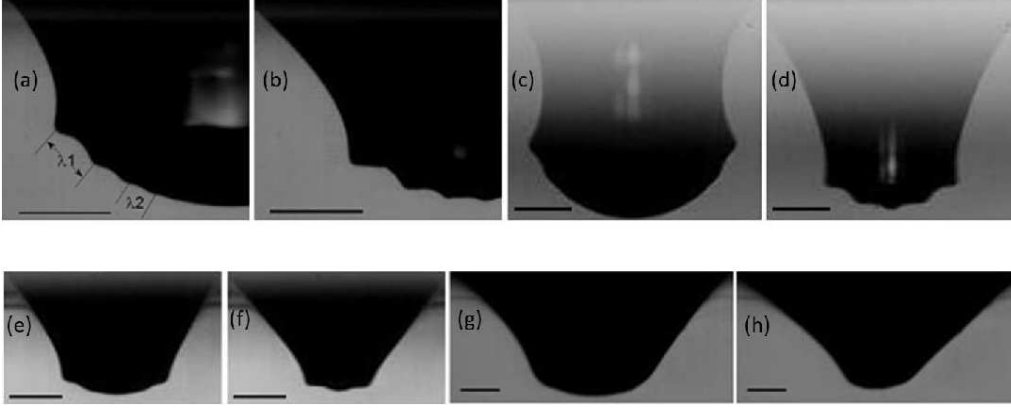
Figure 8: Progressive damping of capillary waves with increase in Oh , shown in image pairs from (a) to (h). Collapsing sequence, (a)-(b): water, Oh = 0.0026 ( Bo = 0.63 ); (c)- (d): water, Oh = 0.0055 ( Bo = 3 \times 10^{-2} ); (e)-(f): GW48 ( 30^\circ C ), Oh = 0.0139 ( Bo = 0.17 ); (g)-(h): GW55, Oh = 0.0225 ( Bo = 0.47 ). In each image pair, images are separated by 741, 100, 148 and 375 micro seconds, respectively. The lines in (a)-(b): 1mm, (c)- (d): 0.2mm, (e)-(f): 0.5mm, (g)-(h):0.5mm.
