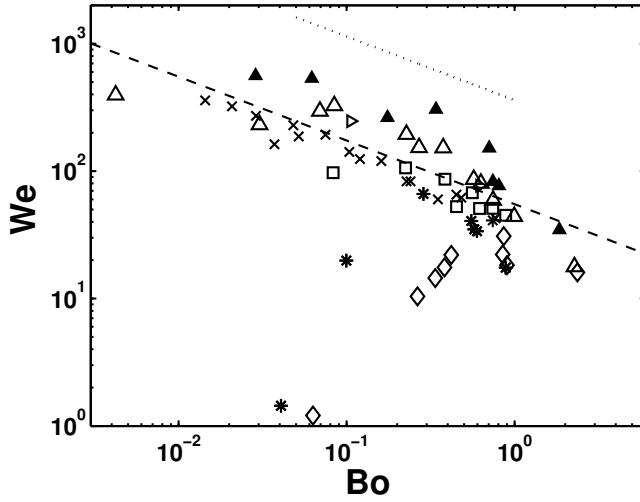
Figure 2: Weber number of the emerging jet velocities as a function of the Bond number. \triangle , Water; \blacktriangle , GW48 (30°C); \triangleright , GW48 (20°C); \square , GW55; * , GW68; \diamond , GW72; \times , the jet velocities of Ghabache et al. (2014) for water; - - , We = 55Bo^{-1/2} ; \dots , the jet velocities of Ghabache et al. (2014) for glycerine-water solutions of viscosities 4.4 to 6.2 mPas.
