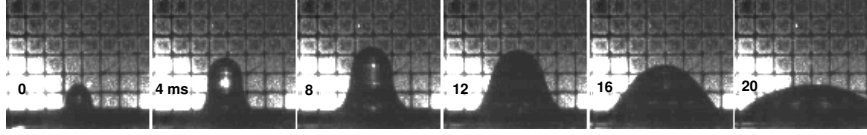
(a) R = 4.08\text{mm} ( Bo = 2.25 , Oh = 1.85 \times 10^{-3} ). The grid size in the image is 1mm. d_j/R \approx 0.32 .
