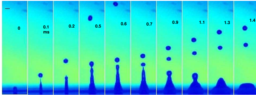
(b) R = 2.15\text{mm} ( Bo = 0.63 , Oh = 2.55 \times 10^{-3} ). The line in image is 1mm. d_j/R \approx 0.24 .
