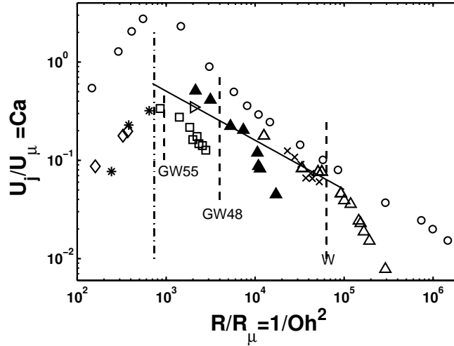
Figure 7: Variation of the dimensionless jet velocity with the dimensionless bubble radius for low Bo . The velocities and radii are normalised by the viscous capillary scales: \triangle , Water; \blacktriangle , GW48 ( 30^\circ C ); \triangleright , GW48 ( 20^\circ C ); \square , GW55; * , GW68; \diamond , GW72; \circ , jet velocities of Duchemin et al. (2002) for water; \times , jet velocities of Ghabache et al. (2014) for water; — , 16(R/R_\mu)^{-1/2} ; -.- , the viscous cut off at R/R_\mu = Oh^{-2} \simeq 730 ; - - , the vertical dashed lines demarcate the Bo < 0.1 data on the left with the Bo > 0.1 data on the right for water (W), GW48 and GW55. Viscous- capillary scaling is seen for Bo < 0.1 part of each data set.
