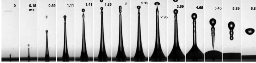
(a) R = 1.04\text{mm} ( Bo = 0.17 , Oh = 1.39 \times 10^{-2} ) in GW48 ( 30^\circ\text{C} ). The line in image is 0.5 mm. d_j/R \approx 0.09 .
