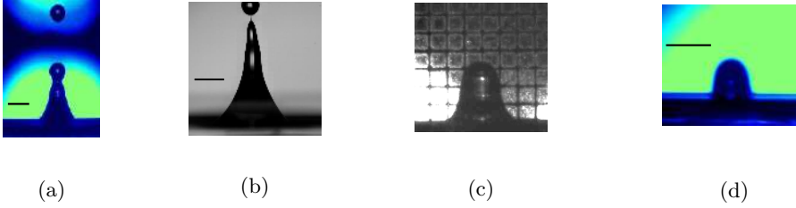
Figure 11: Images of jets for different combinations of Bo and Oh to show the effect of gravity and viscosity. (a) and (b) are at around the same Bo , but (b) has a much larger Oh , still less than Oh = 0.02 . (a) and (c) are at the same Oh < 0.02 , but (c) has a much larger Bo . (a) and (d) have around the same Bo , but (d) has a much larger Oh > Oh_c = 0.037 . (a) Bubble of R = 2.15 mm in water, Bo = 0.629 , Oh = 2.55 \times 10^{-3} ; (b) R = 2 mm in GW48 ( 30^\circ C ), Bo = 0.646 , Oh = 10 \times 10^{-3} ; (c) R = 4.08 mm in water, Bo = 2.25 , Oh = 1.85 \times 10^{-3} ; (d) R = 1.46 mm in GW72, Bo = 0.39 , Oh = 4.9 \times 10^{-2} . The lines in images 11a, 11b and 11d are 1 mm in length. The grid size in image 11c is 1 mm.
