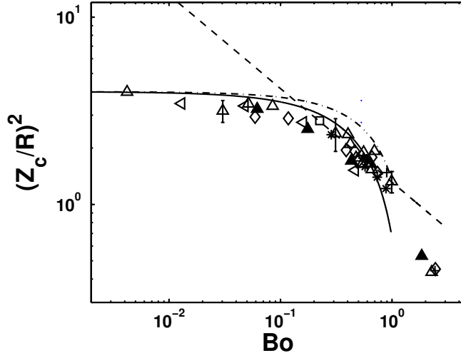
Figure 4: Square of the dimensionless cavity depth of the bubble as a function of the Bond number. \triangle , Water; \triangleright , GW48 (20°C); \blacktriangle , GW48 (30°C); * , GW68; \diamond , GW72; \triangleleft , ethanol; + , 2-propanol; - - , 1.32Bo^{-1/2} ; - \cdot - , (Z_c/R)^2 = 4(1 - 2/3 Bo) ; - , (Z_{cd}/R)^2 = 4(\sqrt{1 - 2/3Bo} - 0.17 Bo^{0.8})^2 .
