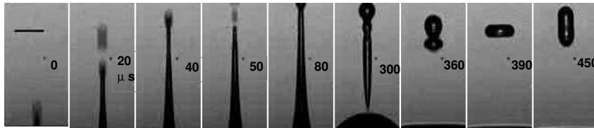
(c) R = 0.71\text{mm} ( Bo = 0.069 , Oh = 4.5 \times 10^{-3} ). The line in image is 0.2mm. d_j/R \approx 0.25 .
