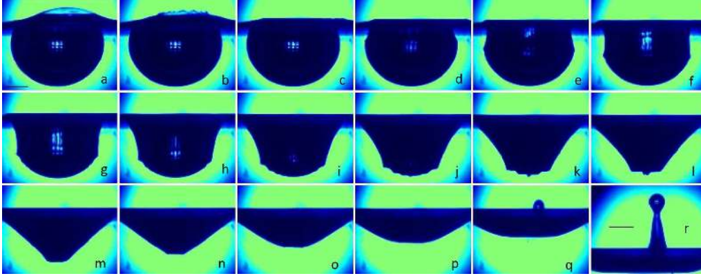
Figure 1: The bursting sequence of a bubble of radius R = 2.15 mm, Bo = 0.63 , Oh = 0.00255 in water. Each image, from a to p, is separated by 0.25 ms. Images p to q and q to r are separated by 0.5 and 1.3 ms respectively. The whole process up to jet emergence at the free surface took 4.5 ms. The lines in images a and r are 1 mm in length.
