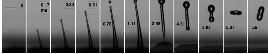
(a) R = 1.04\text{mm} ( Bo = 0.17 , Oh = 1.39 \times 10^{-2} ) in GW48 ( 30^\circ\text{C} ). The line in image is 0.5 mm. d_j/R \approx 0.09 .
