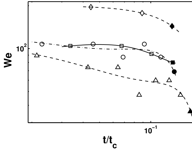
Figure 6: Variation of the jet We with the dimensionless time for bubbles of different Bo in water. \diamond , Bo = 0.2 ; \square , Bo = 0.3 ; \circ , Bo = 0.49 ; \triangle , Bo = 0.63 . Unfragmented jet velocities are shown by hollow symbols while the velocities of the first drop after jet fragmentation are shown by filled symbols. The cubic polynomial fits, show the progression of velocities with time of each jet.
