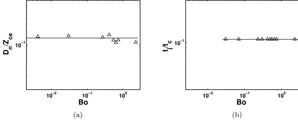
Figure A.13: (a) Variation of the difference between the static cavity depth Z_{ce} and the cavity depth just before jet formation from a conical cavity \tilde{Z}_{ce} , D_n = Z_{ce} - \tilde{Z}_{ce} , in dimensionless form with Bo for water. \Delta , water; —, D_n/Z_{ce} = 0.143 . (b) Variation of the time of cavity retraction measured from the conical shape of the cavity to the jet emergence at the free surface, in dimensionless form, with Bo . —, t_j/t_c = 0.11 .
