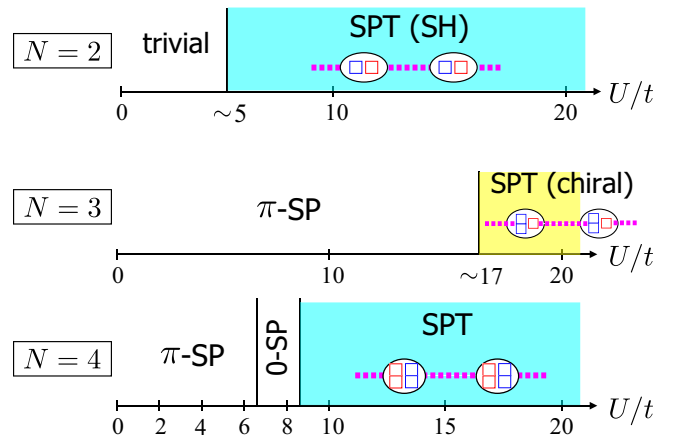
FIG. 4. Phase diagram for N = 2, 3 , and 4 at fixed t_{\perp} = t = 1 , as a function of U (with U/V = 10 ; see the text) obtained from DMRG simulations. In all three cases, we find different SPT phases at strong coupling. For weaker interactions, we find trivial nondegenerate gapped phases, or the out-of-phase (in-phase) dimerized spin-Peierls-like \pi -SP (0-SP) phase.
