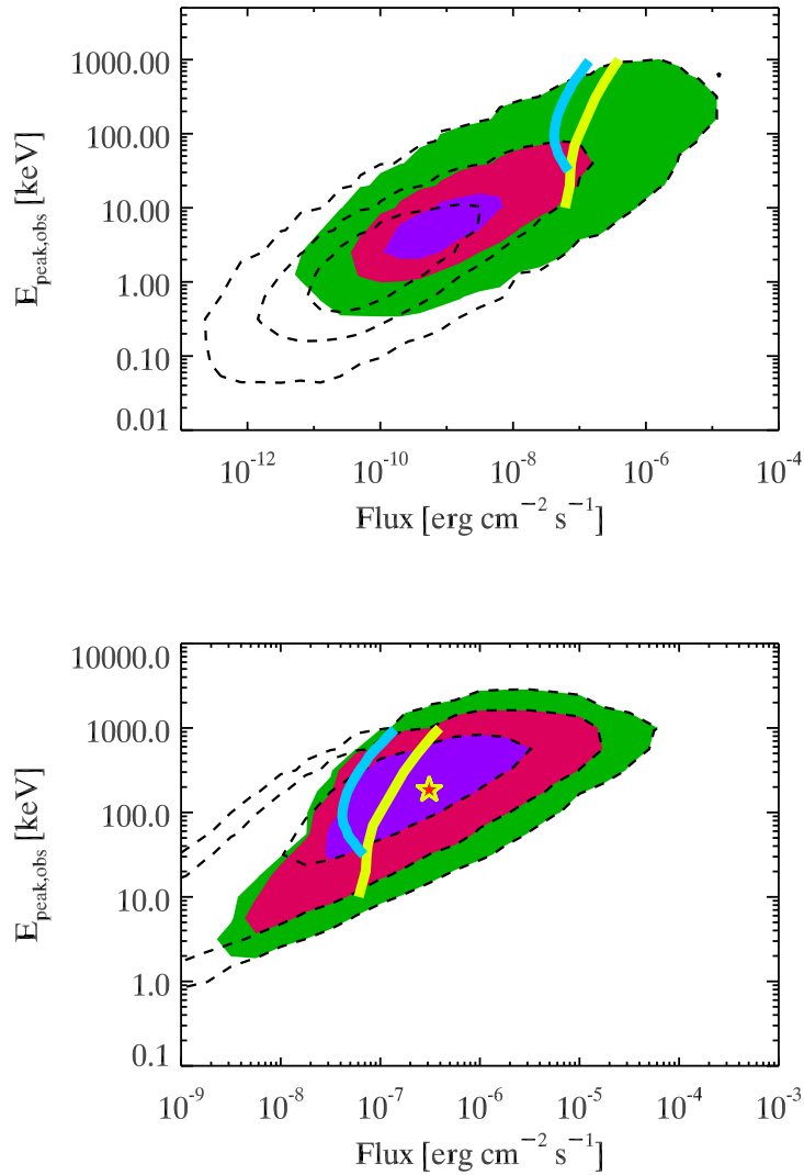
Fig. 4. Density contours (dashed lines) corresponding to 1, 2, 3 \sigma levels of the synthetic population of Long (top) and Short (bottom) GRBs (from Stratta et al. 2017 and references therein). Shaded coloured regions show the density contours of the population detectable by THESEUS. The yellow and cyan lines show the trigger threshold of Fermi/GBM and GCRO/Batse. The flux is integrated over the 10-1000 keV energy range. As can be seen, THESEUS will carry on-board the ideal instruments suite for detecting all classes of GRBs (classical long GRBs, short/hard GRBs, sub-energetic GRBs, and very high-redshift GRBs, which, in this plane, populate the region of weak/soft events), providing a redshift estimate for most of them. The star symbol in the right panel shows the short GRB170817A associated with the NS-NS gravitational-wave event GW170817. As can be seen, THESEUS will be capable of detecting and localizing substantially weaker and softer events with respect to, e.g., the Fermi/GBM, thus granting the detection of short GRBs associated to NS-NS or NS-BH merger events up to a much larger horizon.
