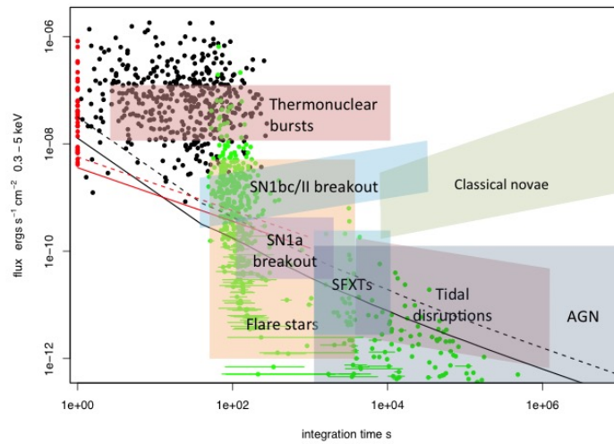
Fig. 3. Sensitivity of the SXI (black curves) and XGIS (red) vs. integration time (Amati et al. 2017). The solid curves assume a source column density of 5 \times 10^{20} \text{ cm}^{-2} (i.e., well out of the Galactic plane and very little intrinsic absorption). The dotted curves assume a source column density of 10^{22} \text{ cm}^{-2} (significant intrinsic absorption). The black dots are the peak fluxes for Swift BAT GRBs plotted against T_{90}/2 (where T_{90} is defined as the time interval over which 90% of the total background-subtracted counts are observed, with the interval starting when 5% of the total counts have been observed). The red dots are those GRBs for which T_{90}/2 is less than 1 s. The green dots are the initial fluxes and times since trigger at the start of the Swift XRT GRB light-curves. The horizontal lines indicate the duration of the first time bin in the XRT light-curve. The various shaded regions illustrate variability and flux regions for different types of transients and variable sources.
