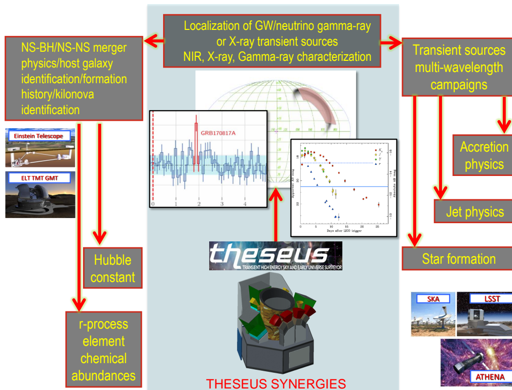
Fig. 8. Expected impact of THESEUS on multi-messenger and time domain astronomy (see Amati et al. 2017 and Stratta et al. 2017 for credits and references of the figures composing this sketch). THESEUS will have the unique capability of monitoring the X/soft gamma-ray sky with a FOV as large as the current “only-LIGO” error regions for GW events (such large regions may be expected also in the future for the farthest events that may be detected only by the most sensitive GW detector) with source location accuracy down to 0.5' and unprecedented sensitivity. Moreover, its payload will be perfectly suited to detect, accurately locate (down to 1'' ) and measure the redshift of all classes of GRBs, including short GRBs, the most relevant for multi-messenger astrophysics. Thus, for NS-NS and NS-BH events like GW170817, THESEUS will have the possibility of detecting and localizing to a few arcmin the associated short GRB, of providing detection, 1 arcsec localization and redshift of the associated NIR kilonova emission and even of detecting the possible soft X-ray emission associated to the merger predicted by several models. More in general, THESEUS will be an unprecedentedly powerful transients machine, thus providing a unique synergy and complementarity with the large multi-wavelength observatories of the future (e.g., E-ELT, TMT, SKA, CTA, ATHENA) and a substantial contribution to time-domain astronomy.
