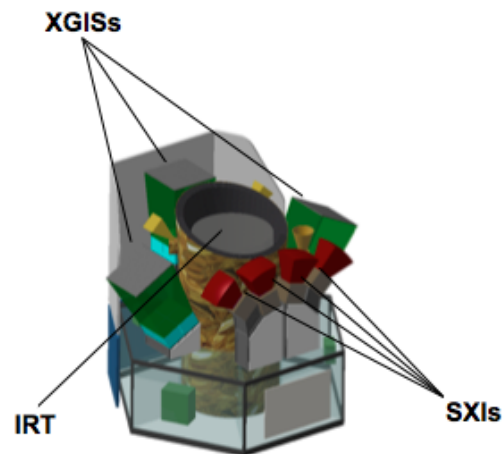
Fig. 1. THESEUS Satellite Baseline Configuration and Instrument suite accommodation (Amati et al. 2017)
