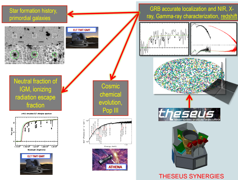
Fig. 7. Expected impact of THESEUS of early Universe science, also in synergy with large observing facilities of the near future like, e.g., E-ELT, TMT, ATHENA (see Amati et al. 2017 and Stratta et al. 2017 for credits and references of the figures composing this sketch). THESEUS (will provide a substantial step forward in the detection, accurate localization and redshift measurements of high- z GRBs ( \sim 20\text{--}40 at z \lesssim 8 and \sim 75\text{--}150 at z \lesssim 6 in 4 years of operations) and use its own measurements for getting unique clues to the first population of stars (pop III) and galaxies, the sources and evolution of the re-ionization process, SFR history and galaxy metallicity evolution up to the end of the dark ages and their interplay. However, for very high- z GRBs (e.g., z > 8 ), follow-up observations (deep spectroscopy of the afterglow, imaging and spectroscopy of the host galaxy) by very large and extremely large telescopes, will provide an important contribution in fully exploiting THESEUS measurements for early Universe science. Remarkable will be also the synergy with the future large X-ray observatory ATHENA. Indeed, THESEUS, by providing real time triggers, accurate location and redshift of GRBs over the whole cosmic history and up z \lesssim 10\text{--}12 , will enable ATHENA to achieve some of its main goals: high-resolution X-ray spectroscopy of bright GRBs afterglow to probe the Warm Hot Intergalactic Medium (the WHIM) and hence get clues to the missing baryons problem; probe the first generation of stars through the study of the circum-burst environment. Many of the other transients found by THESEUS, such as tidal disruption events and flaring binaries will also be high-value targets for Athena
