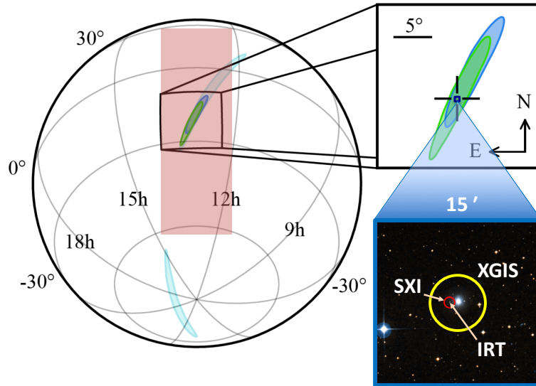
Fig. 6. The plot (Stratta et al. 2017 and references there in) shows the THESEUS/SXI field of view ( \sim 110 \times 30 \text{ deg}^2 , pink rectangle) superimposed on the probability skymap of GW 170817 obtained with the two Advanced LIGO only (cyan) and with the addition of Advanced Virgo (green). THESEUS not only will cover a large fraction of the skymap (even those obtained with only two GW-detectors, e.g. cyan area), but will also localize the counterpart with uncertainty of the order of 5 arcmin with the XGIS and to less than 1 arcmin with SXI. The THESEUS location accuracy of GW events produced by NS-NS mergers can be as good as 1 arcsec in case of detection of the kilonova emission by the IRT. By the end of the 2020s, if ET will be a single detector, almost no directional information will be available for GW sources ( > 1000 \text{ deg}^2 for BNS at z > 0.3 and a GRB-localising satellite will be essential to discover EM counterparts.
