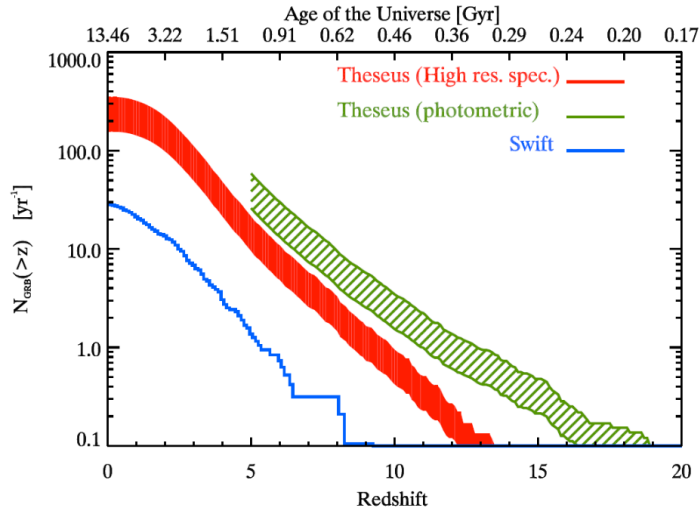
Fig. 2. The yearly cumulative distribution of GRBs with redshift determination as a function of the redshift for Swift and THESEUS (Amati et al. 2017). The THESEUS expected improvement in the detection and identification of GRBs at very high redshift w/r to present situation is impressive (more than 100–150 GRBs at z > 6 and several tens at z > 8 in a few years) and will allow the mission to shed light on main open issues early Universe science (star formation rate evolution, re-ionization, pop III stars, metallicity evolution of first galaxies, etc.).
