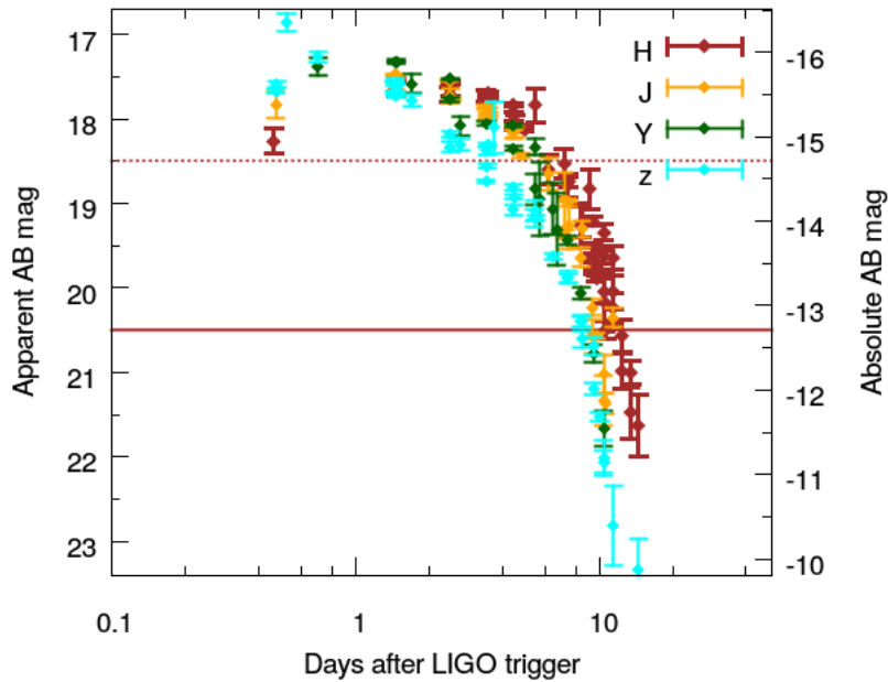
Fig. 5. Light curve of the kilonova associated to the gravitational wave/short GRB event GW170817/GRB170817A in the IRT filters (Stratta et al. 2017 and references therein). The continuous and dashed red lines indicate the THESEUS/IRT limiting H magnitudes for imaging and prism spectroscopy, respectively, with 300s of exposure (see Amati et al. 2017).
