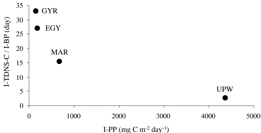
Fig. 4. Relationship between I-TDNS-C/I-BP ratios [total dissolved neutral sugars in carbon integrated down to DCM (I-TDNS-C in mg C m -2 ) and bacterial production integrated down to DCM (I-BP in mg C m -2 day -1 )] and primary production integrated down to DCM (I-PP in mg C m -2 day -1 ) at the four stations in the South East Pacific.
