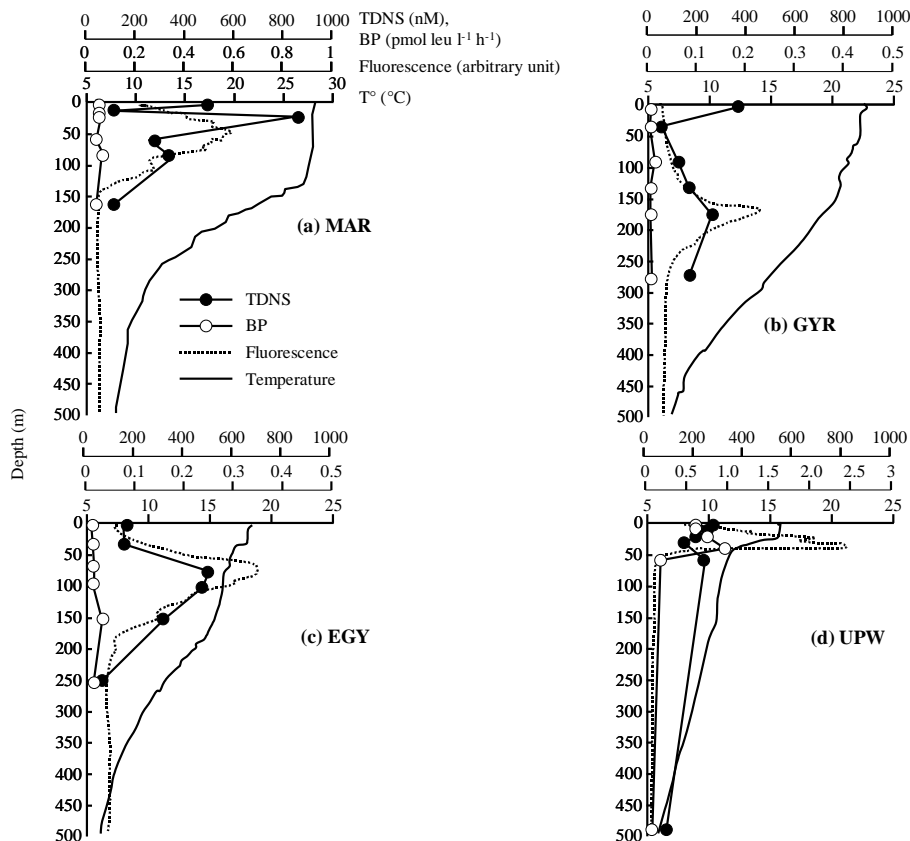
Fig. 2. Depth profiles of total dissolved neutral sugars (TDNS in nM), bacterial production (BP in \text{pmol leu l}^{-1} \text{h}^{-1} ), chlorophyll fluorescence (arbitrary unit), and temperature ( ^{\circ}\text{C} ) at the four stations in the South East Pacific.
