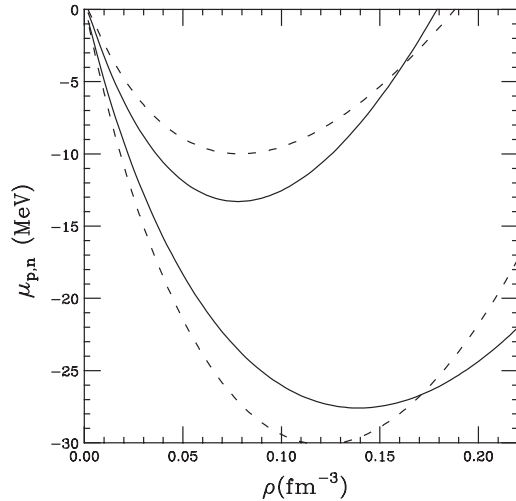
Fig. 4. Density dependence, for I=0.2 , of neutron (upper curves) and proton (lower curves) chemical potentials for asy-superstiff ( \gamma \sim 1.6 - solid lines) and asy-soft ( \gamma=0.5 - dashed lines) EOS. From [32].
