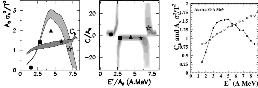
Fig. 37. Left panel: normalized kinetic energy fluctuations and estimated C_k values for quasi-projectile events produced in Au+Au collisions at 35 MeV per nucleon (grey zones) and for fused systems produced in central Au+C (black dots), Au+Cu (squares, triangles) and Au+Au reactions before (open stars) and after subtraction of 1 MeV per nucleon radial flow (black stars). Central panel: corresponding microcanonical heat capacities per nucleon. Grey zones indicate confidence regions. From [218]. Right panel: normalized kinetic energy fluctuations (filled circles) and estimated C_k values (open circles) for quasi-projectile events produced in Au+Au collisions at 80 MeV per nucleon. From [219].
