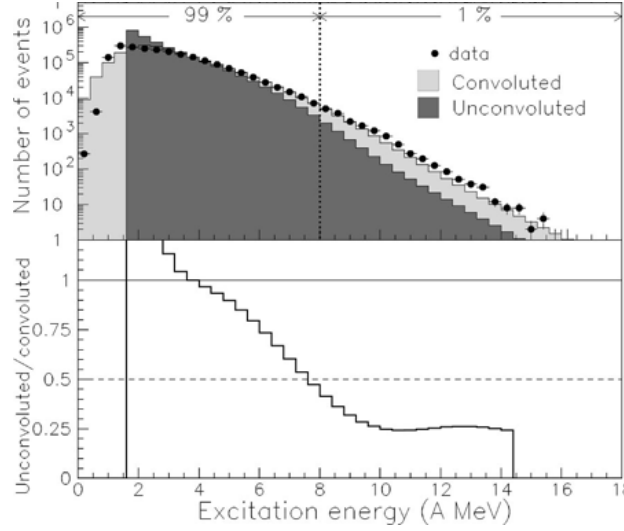
Fig. 20. Top : Convolved, unconvolved and experimental excitation energy distributions obtained in \pi +Au reactions. Bottom : Ratio of unconvolved-to-convolved distribution as a function of the excitation energy per nucleon. Adapted from [173]
