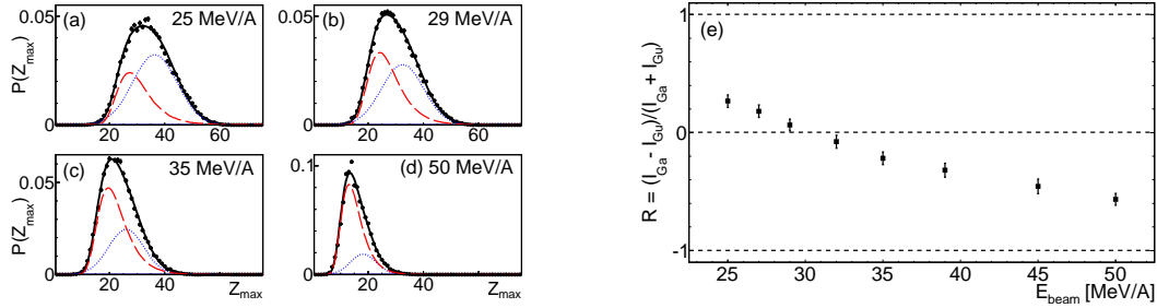
Fig. 42. (a)-(d): Charge distributions of the largest fragment of each event Z_{max} in central quasifusion collisions of Xe on Sn at the bombarding energies shown. Data: points; black line: fit of the distribution with an admixture of gaussian and gumbellian distributions; red dashed line: gumbellian component; blue dotted line: gaussian component. (e) Relative strengths of the two components, R (see Eq. (31)), as a function of the beam energy. Adapted from [253].
