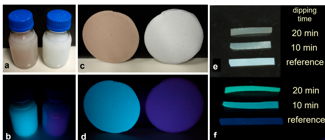
Figure 6. Aqueous suspensions of TEMPO-mediated oxidation and nanofibrillation of bacterial cellulose (TOBC) nanofibrils covalently equipped with GEA-type CDs (a,b) and nanopaper prepared therefrom (c,d) at daylight (a,c) and UV excitation (the CD-free reference material is shown in each of the pictures a-d on the right). Pictures of prefabricated TOBC nanopaper subjected to EDC/NHS-mediated dip-grafting of GEA-type CDs (10 or 20 min) taken at daylight (e) or under UV light (f).
