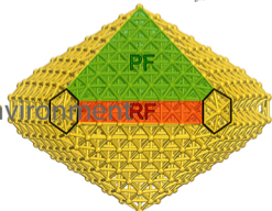
Marks-decahedron ( D_{5h} )
