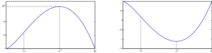
FIGURE 5. Graphs of the functions h (left) and \psi (right) for r = 0.3 , K = 5 , \alpha = 2.5 , E_{max} = 0.5893 , E^* = 0.6235 .
