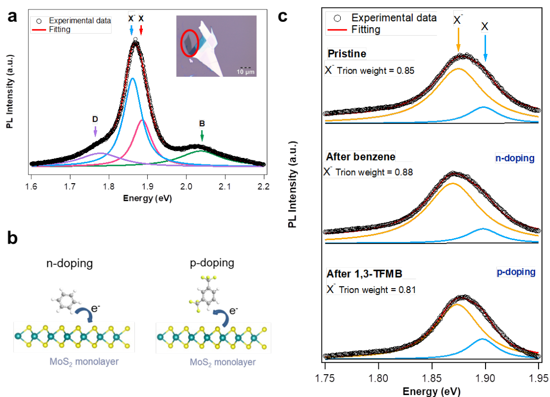
Figure 1. a) Photoluminescence spectra of monolayer MoS 2 at 78 K (inset: optical image of as exfoliated monolayer MoS 2 highlighted with a red circle). b) Molecular representation of charge transfer between physisorbed aromatic molecules and monolayer MoS 2 . c) Photoluminescence spectra of monolayer MoS 2 before and after physisorption of benzene and 1,3-TFMB with calculated X - trion weight.
